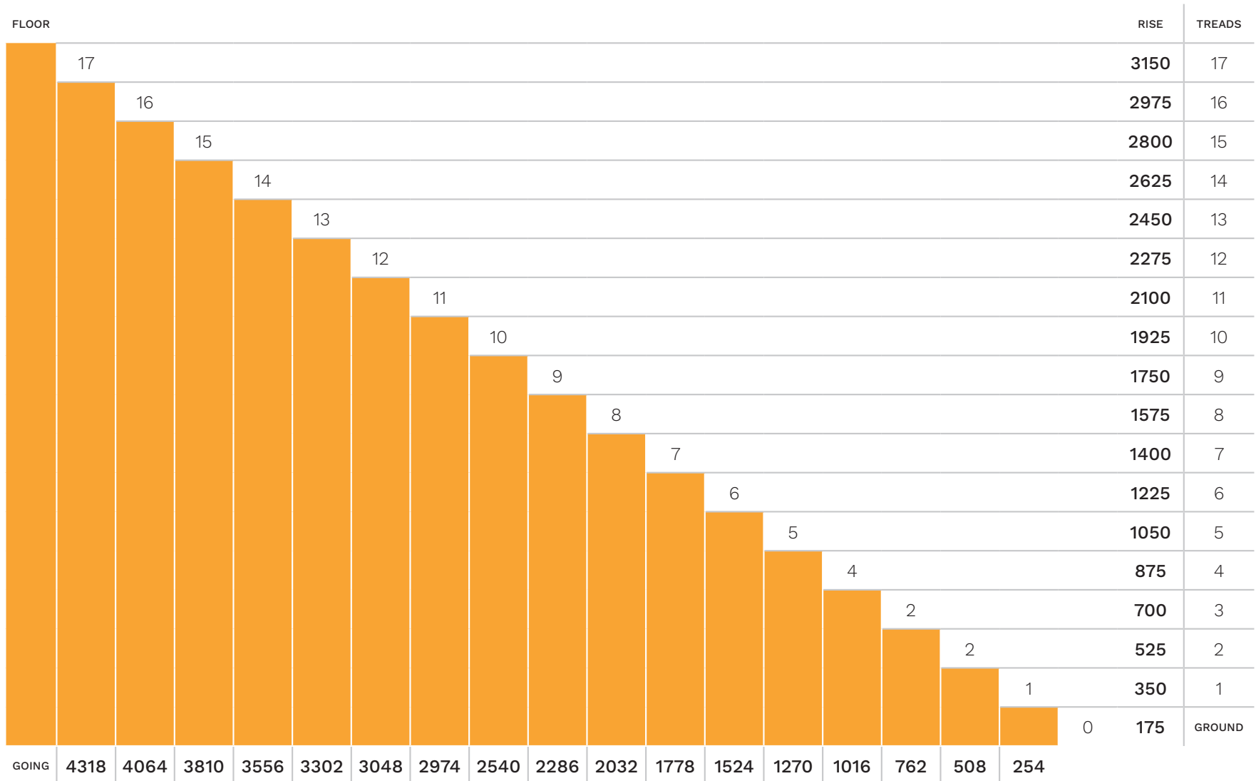
Stair Stringers - Made to Suit 175mm Rise with a Going of 254mm
